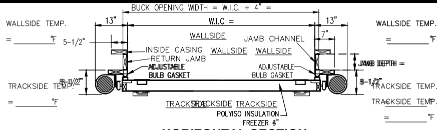
HORIZONTAL SECTION
