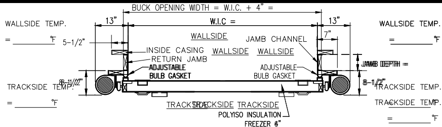
HORIZONTAL SECTION
