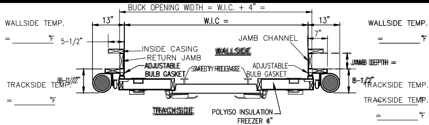
HORIZONTAL SECTION
